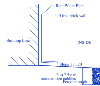
PERCOLATION PIT
