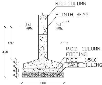
FOUNDATION DETAIL
