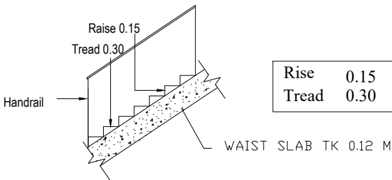
STAIRCASE DETAIL
