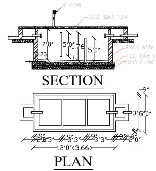
PLAN SEPTIC TANK DETAILS
