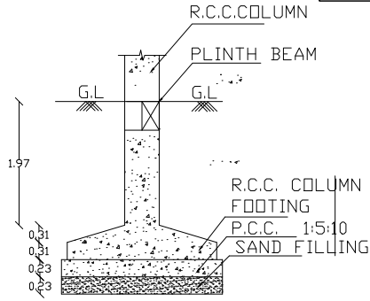
FOUNDATION DETAIL
