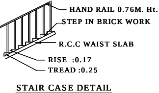
STAIR CASE DETAIL
