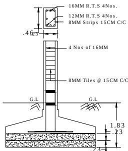
RCC COLUMN DETAILS
