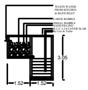
RECYCLING OF WASTE WATER FROM KITCHEN & BATHROOM
