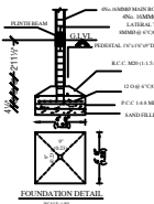
FOUNDATION DETAILS
