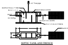
SEPTIC TANK AND TRENCH
