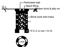
PERCOLATION PIT FOR 30 Sq.m (NOT FOR SCALE)
