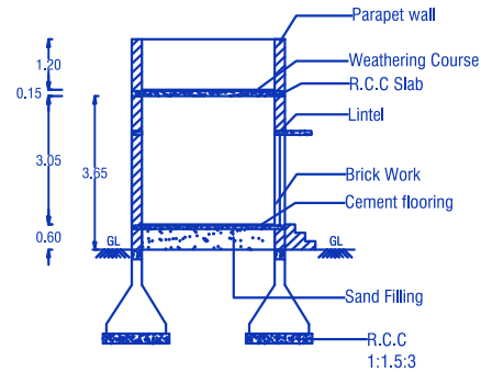
CROSS SECTION ON 'AB'
