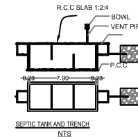
SEPTIC TANK AND TRENCH NTS
