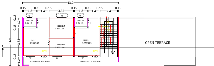
SECOND FLOOR PLAN(HEAD ROOM)
