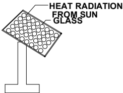
SOLAR SYSTEM
