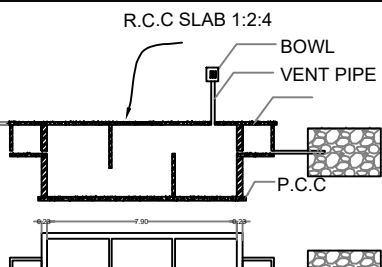
SEPTIC TANK AND TRENCH NTS
