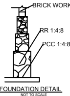
FOUNDATION DETAIL
