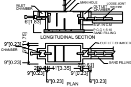
SEPTIC TANK:
