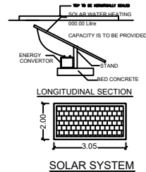
SOLAR SYSTEM
