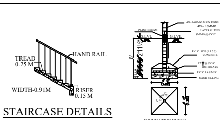
STAIRCASE DETAILS
