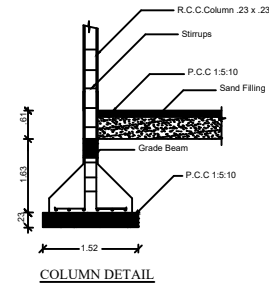
COLUMN DETAIL
