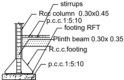
COLUMN DETAILS
