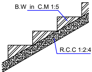
STAIRCASE
