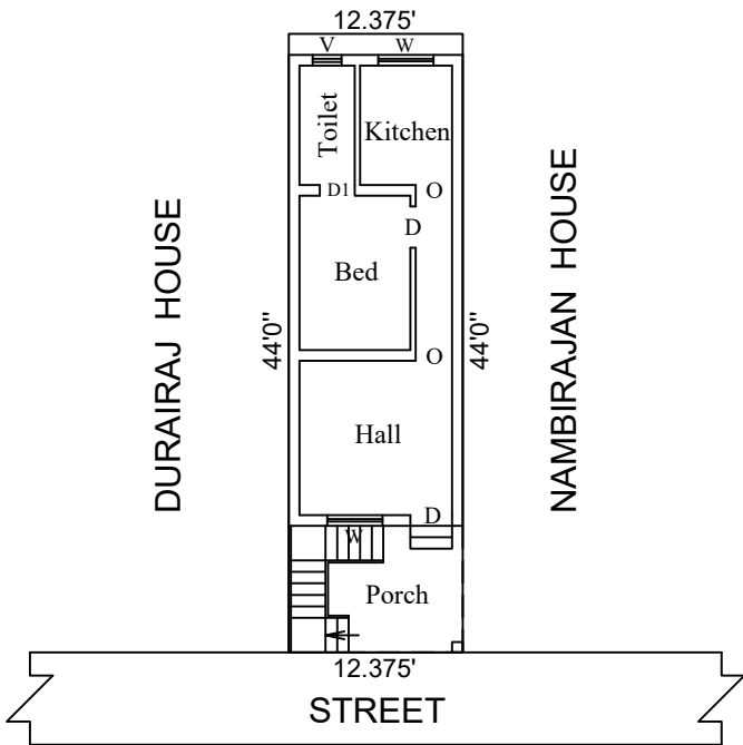
SITE PLAN
