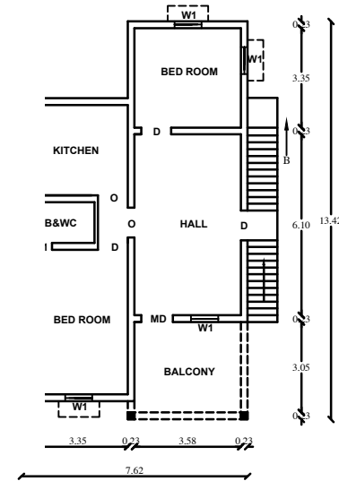
PRO FIRST FLOOR PLAN SCALE:1:100
