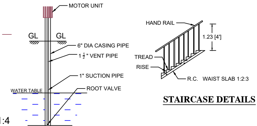
SEC.OF BOREWELL
