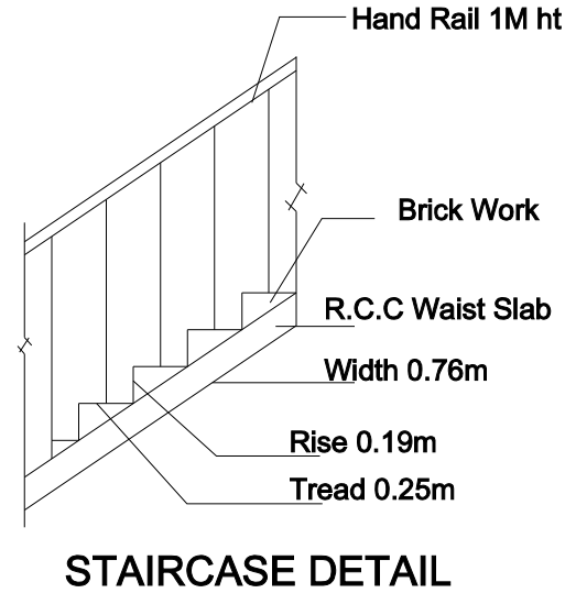
STAIRCASE DETAIL
