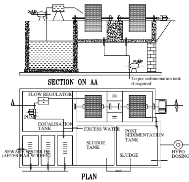
SEWAGE TREATMENT PLANT DETAILS WASTE WATER RECYCLING UNIT
