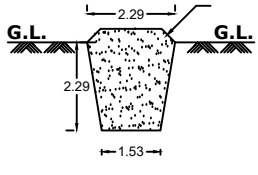
TRIAL PIT (Scale 1:100)
