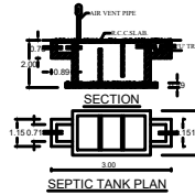
SEPTIC TANK PLAN
