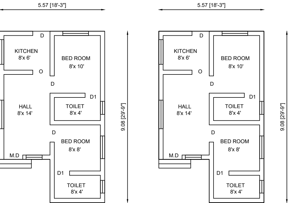
PLAN - A
