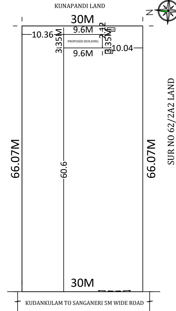
SITE PLAN 1:500 SCALE
