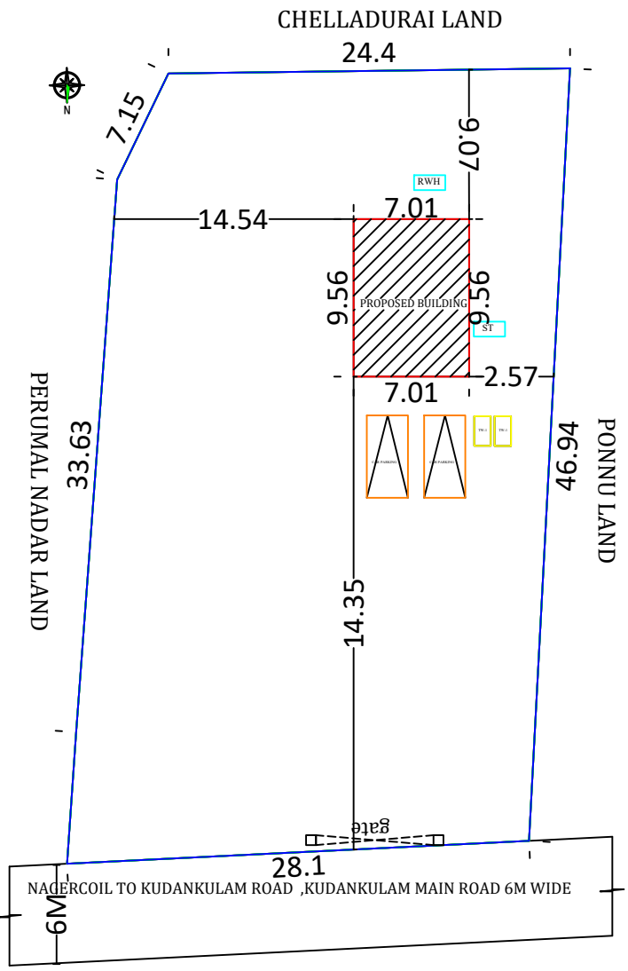
SITE PLAN 1:200 SCALE
