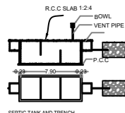
SEPTIC TANK AND TRENCH NTS
