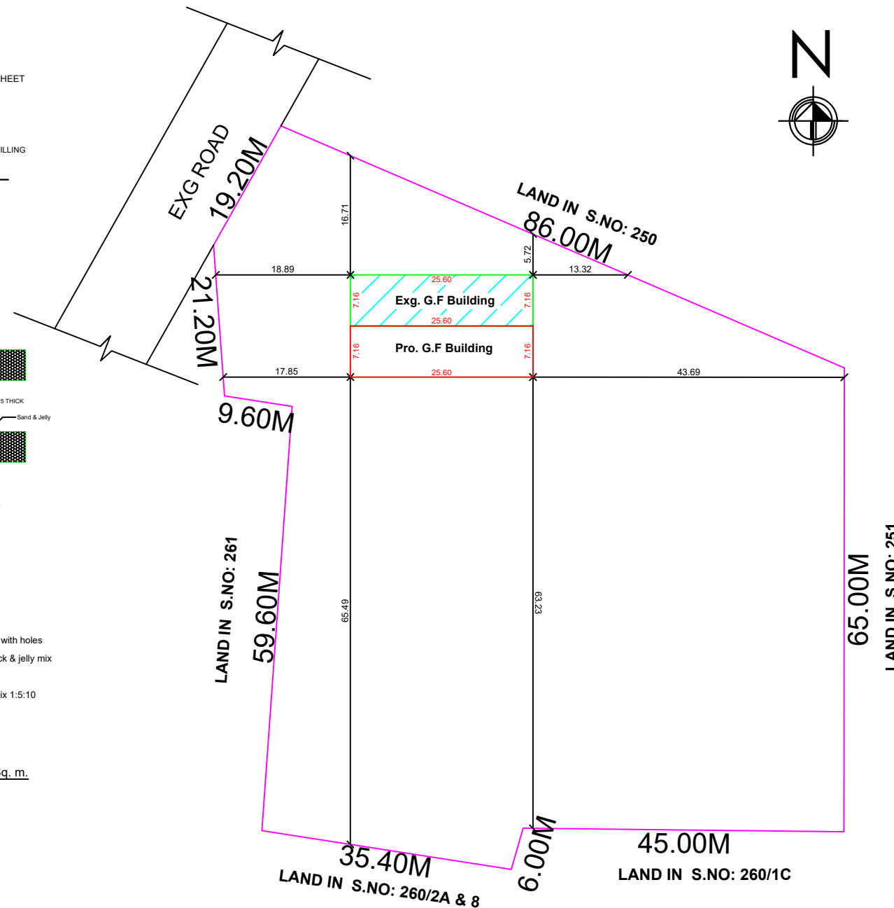
SITE PLAN (SCALE:1:400)
