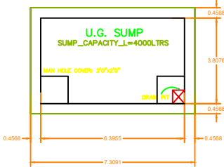
SUMP DETAIL SCALE 1"=4'0"
