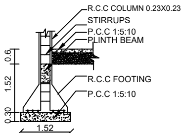
COLOUMN DETAILS
