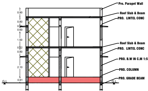
CROSS SECTION ON XX
