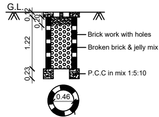
PERCOLATION PIT FOR 30 Sq. m. (Scale:- 1:50)
