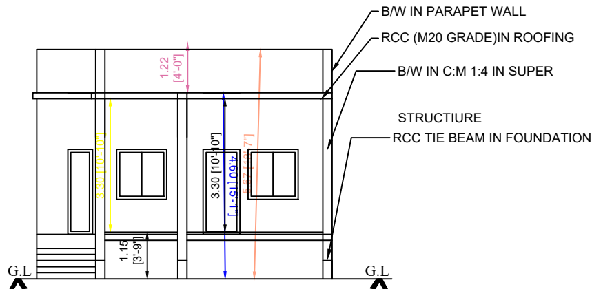
SECTION AA
