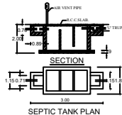
SEPTIC TANK PLAN
