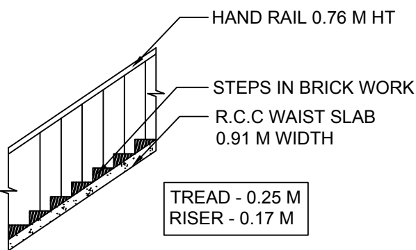
STEP DETAILS
