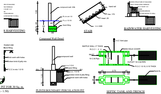
PLINTH BOUNDARY PERCOLATION PIT
