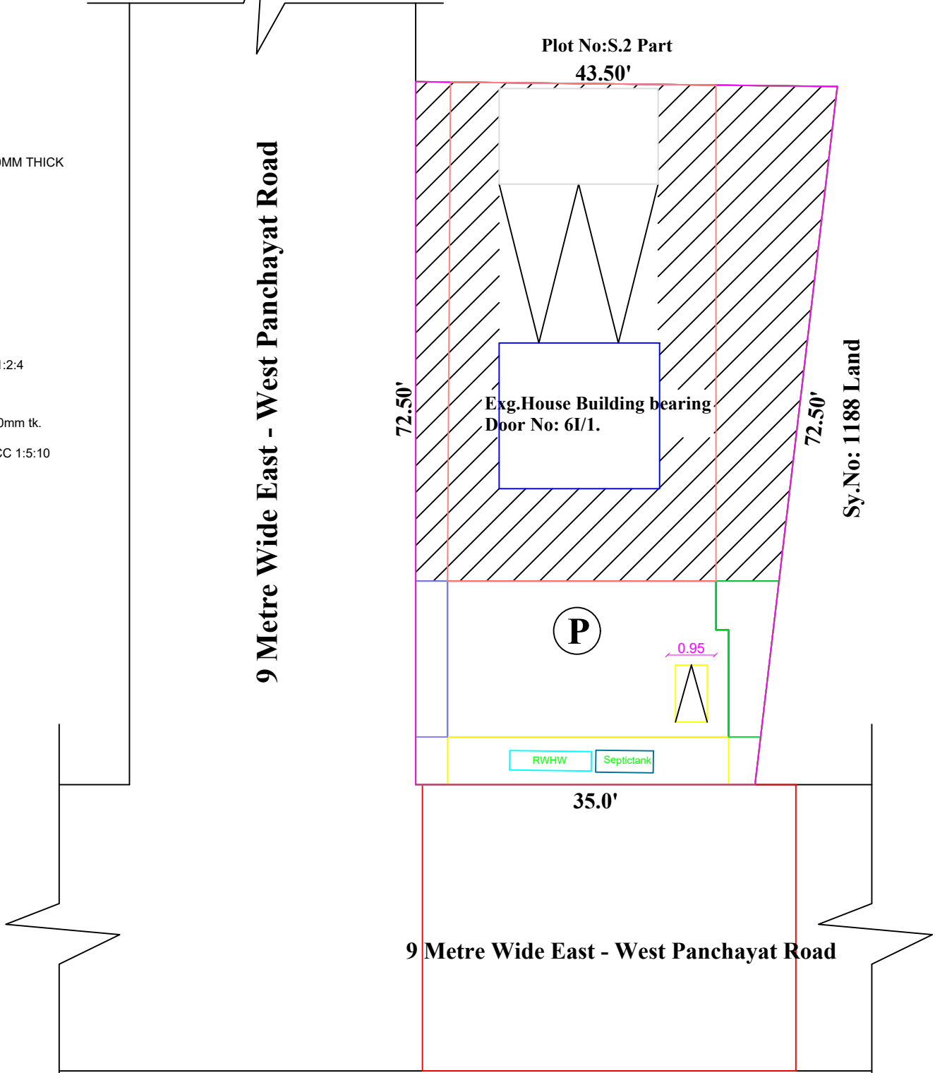
SITE PLAN
