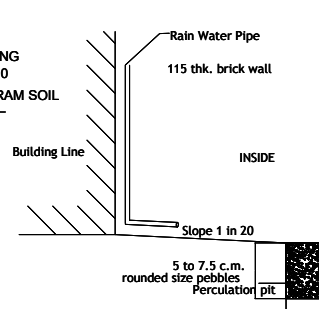
PERCOLATION PIT
