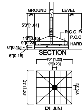
FOUNDATION DETAILS
