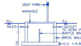
SECTION OF SEPT. TANK
