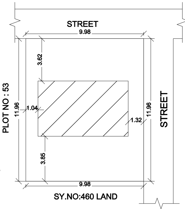
SITE PLAN
