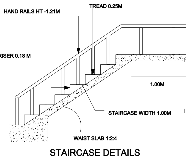
STAIRCASE DETAILS
