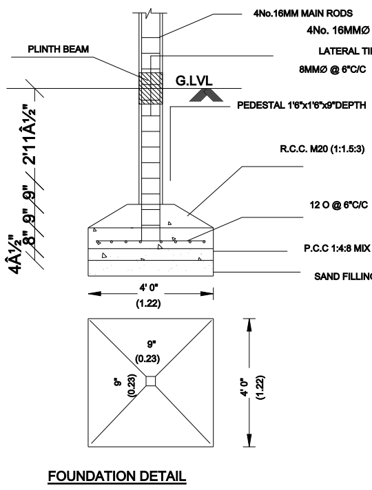
FOUNDATION DETAIL
