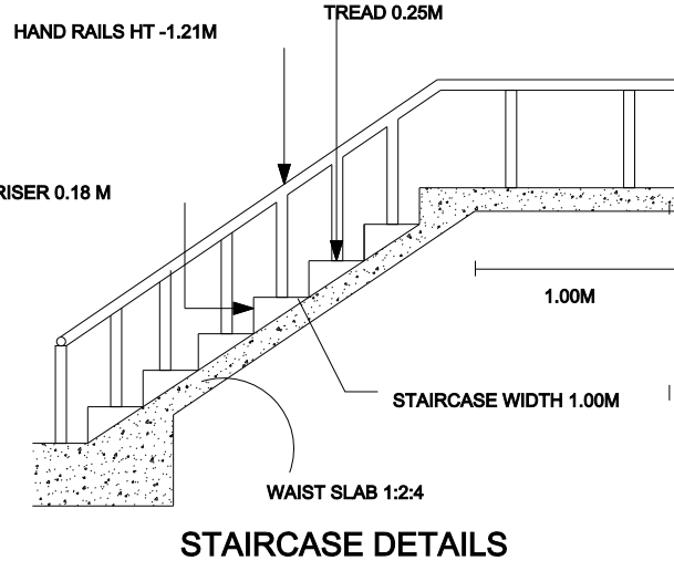
STAIRCASE DETAILS
