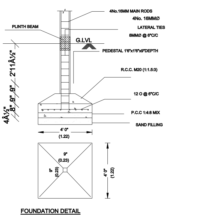
FOUNDATION DETAILS
