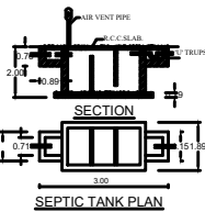
SEPTIC TANK PLAN
