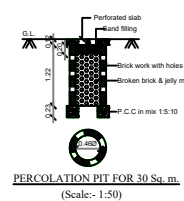
RAINWATER HARVESTING
