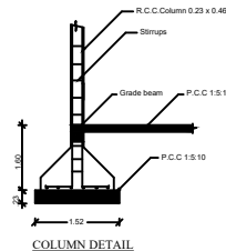
COLUMN DETAIL
