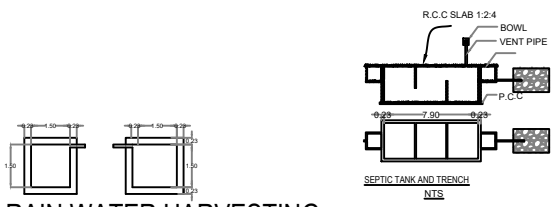
RAIN WATER HARVESTING NTS
