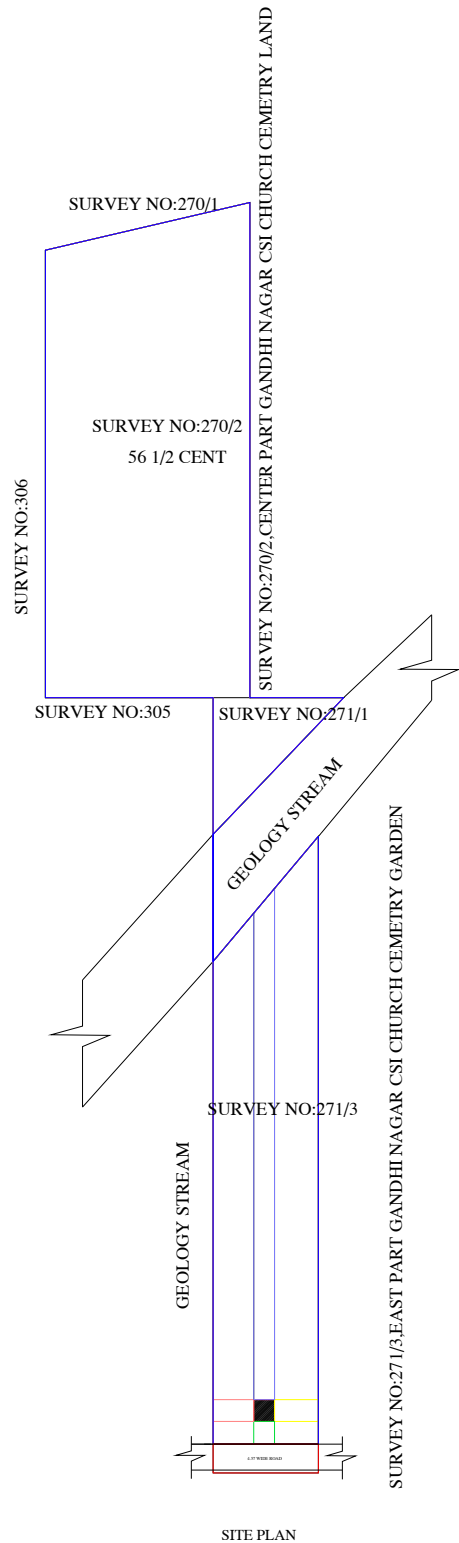
SITE PLAN
