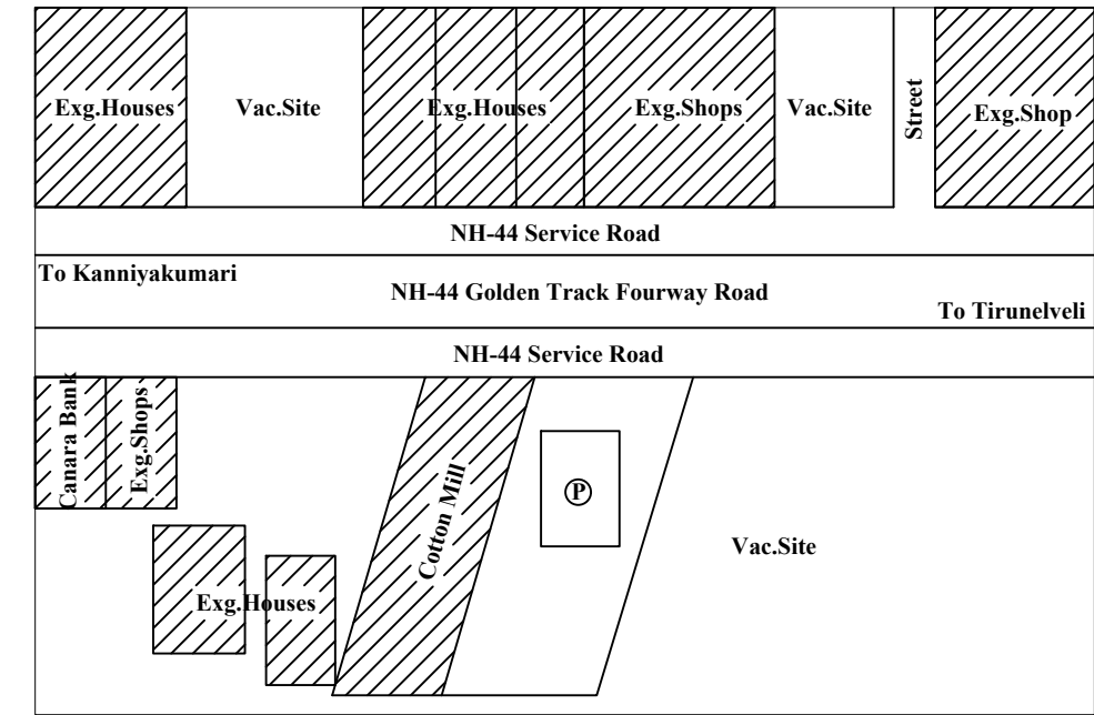
LOCATION PLAN
