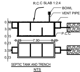
SEPTIC TANK AND TRENCH NTS
