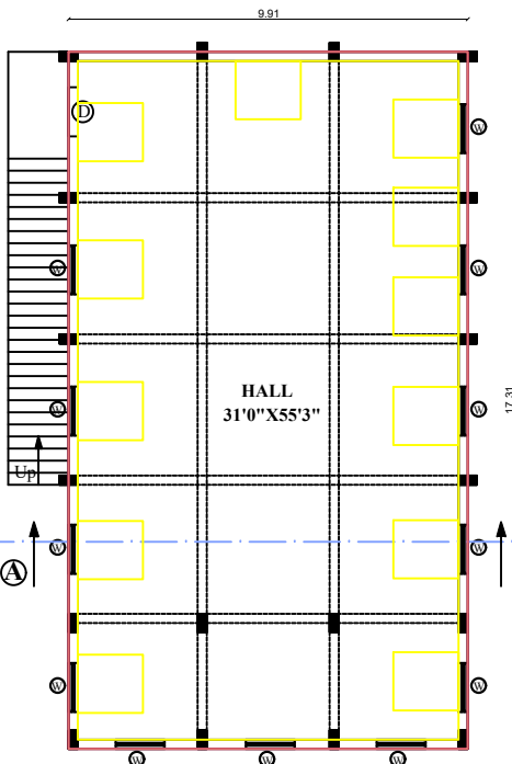
PRO. FIRST FLOOR PLAN
