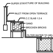
DETAILS OF FILTER BED & WELL NTS
