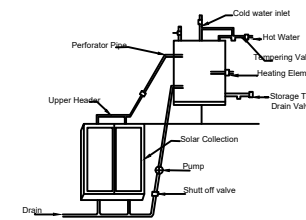
Details Of Solar Water Heater (NTS)
