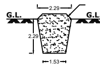
TRIAL PIT (Scale 1:100)
