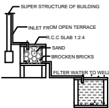
DETAILS OF FILTER BED & WELL
