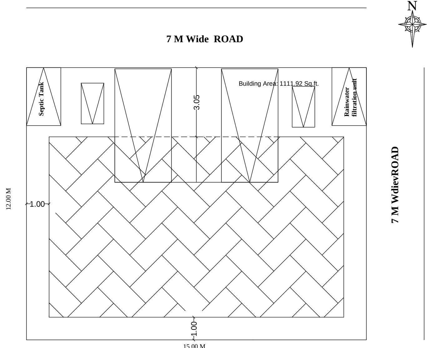
PLAN OF SEPTIC TANK & TRENCH
