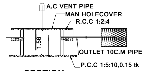
PLAN & SECTION OF RAIN WATER COLLECTION WELL
