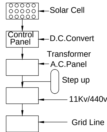
SOLAR SYSTEM
