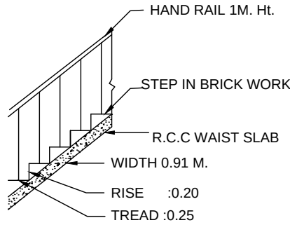
STAIR DETAIL
