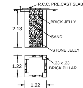
PLAN & SECTION OF RAIN WATER COLLECTION WELL
