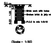
PERCOLATION PIT FOR 30 Sq. m.
