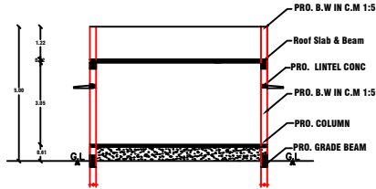
CROSS SECTION ON XX
