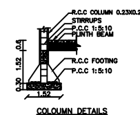
COLUMN DETAILS
