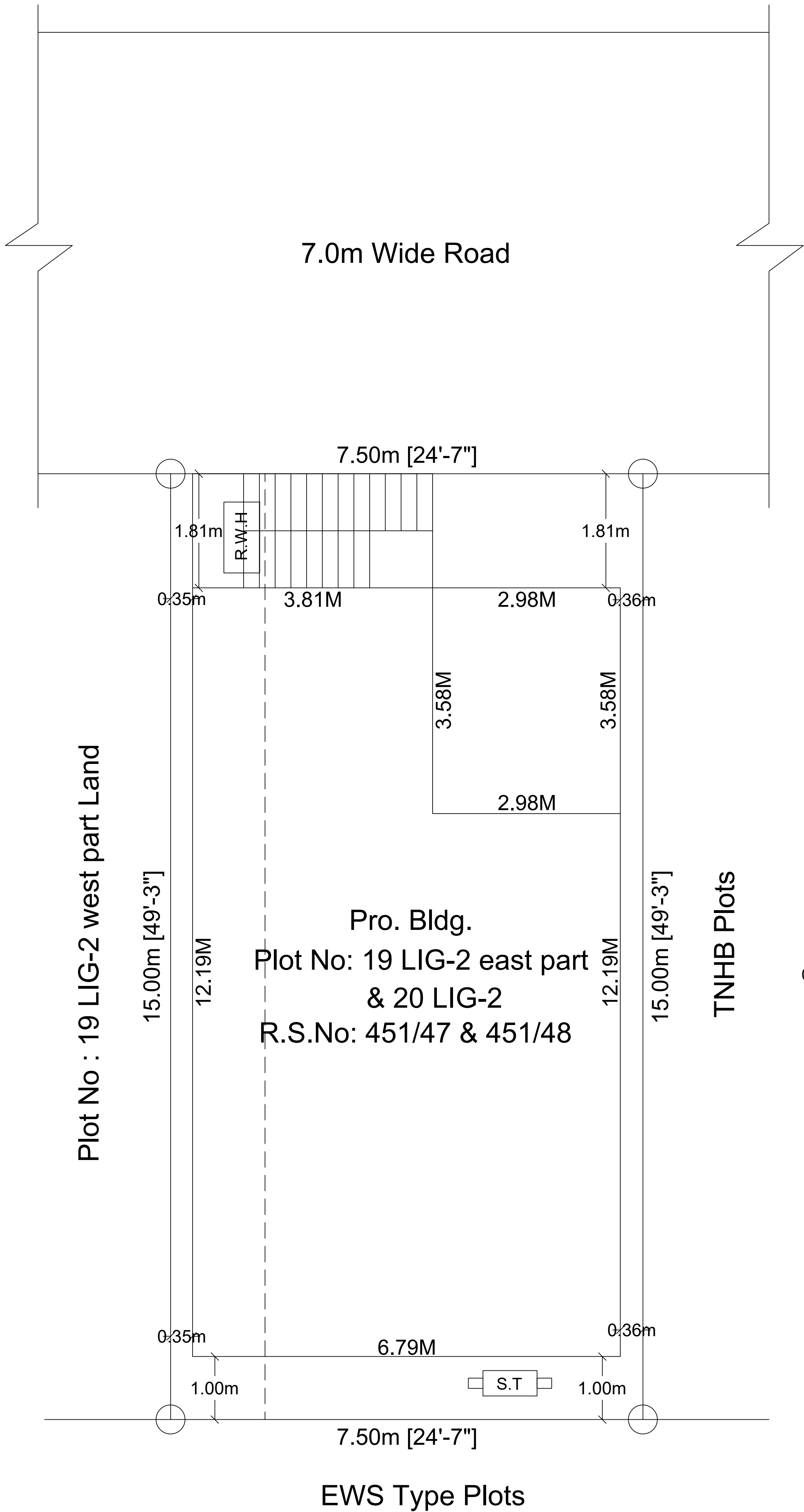
SITE PLAN
