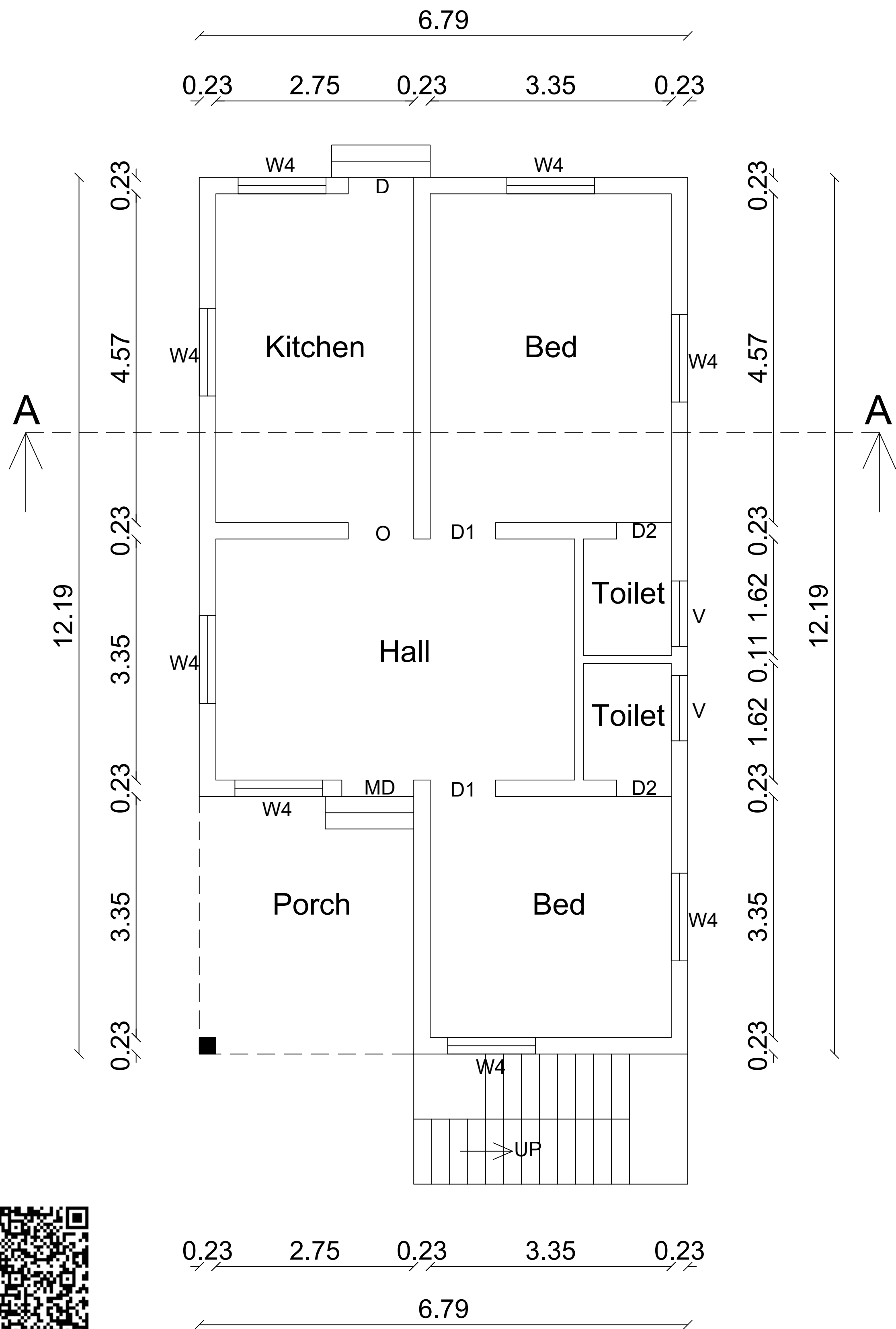
PLAN
