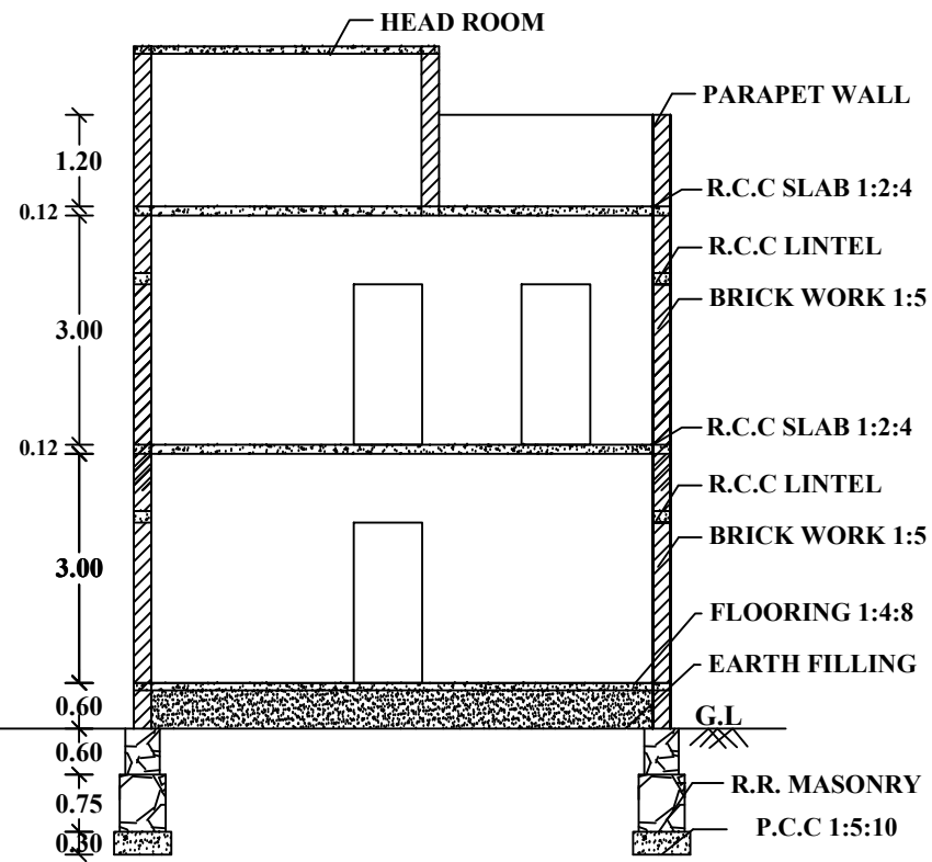
SECTION "AB"
